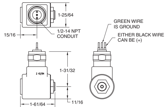
Classic Style “Mold-Over” Solenoid Operator
