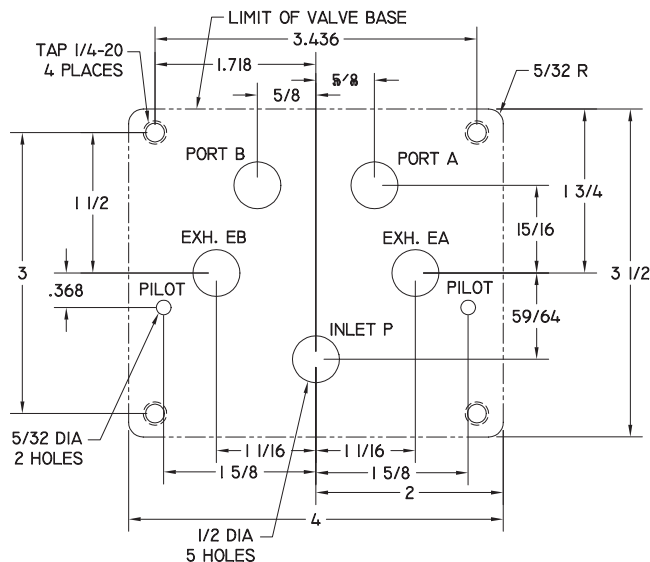
MOUNTING PATTERN — 1/2" VALVES
