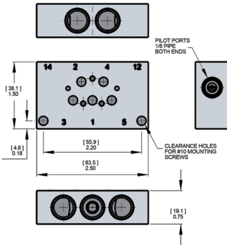
DASH 3 1/4 PIPE SIDE PORTED 1/4 NPT B03N2S 1/4 BSPP B03B2S
