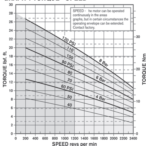
GRAPH 1 TORQUE - SPEED
