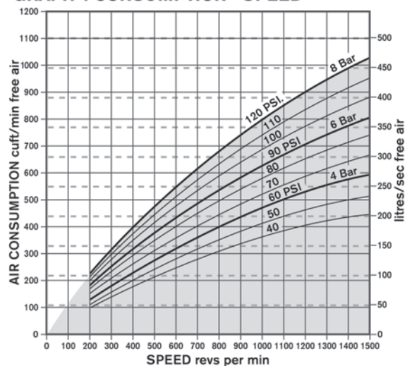
GRAPH 4 CONSUMPTION - SPEED
