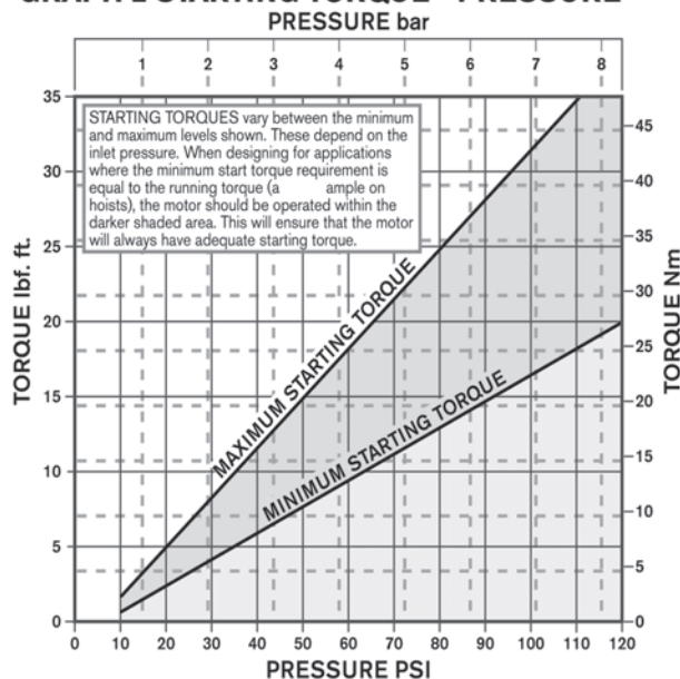
GRAPH 2 STARTING TORQUE - PRESSURE
