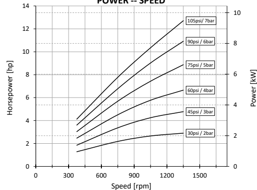
POWER -- SPEED
