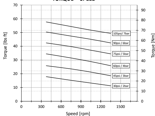
TORQUE -- SPEED
