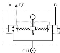
CIRCUIT SYMBOL LEVER CONTROL VALVE
