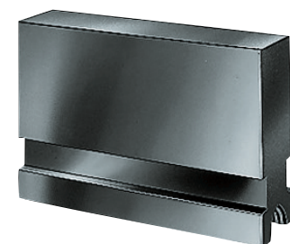
Unstepped jaw BL, unstepped, soft, material 16MnCr5
