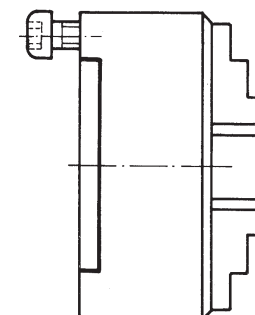
A09 DIN 6351, cylindrical centre mount, form A
