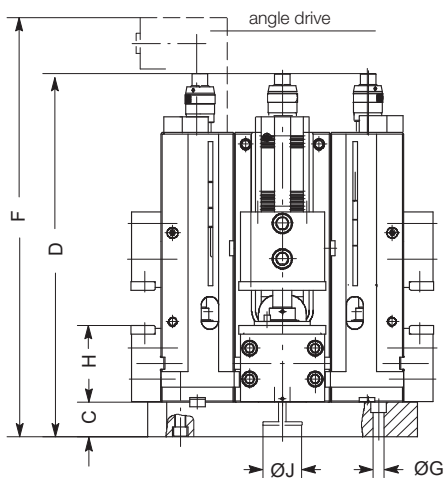
Quattro-clamping towers (on request)
