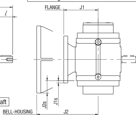
Vers.5: Vers.1 with bell-housing and coupling IEC
