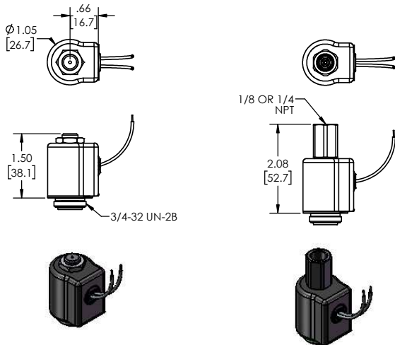
GROMMET HOUSING
