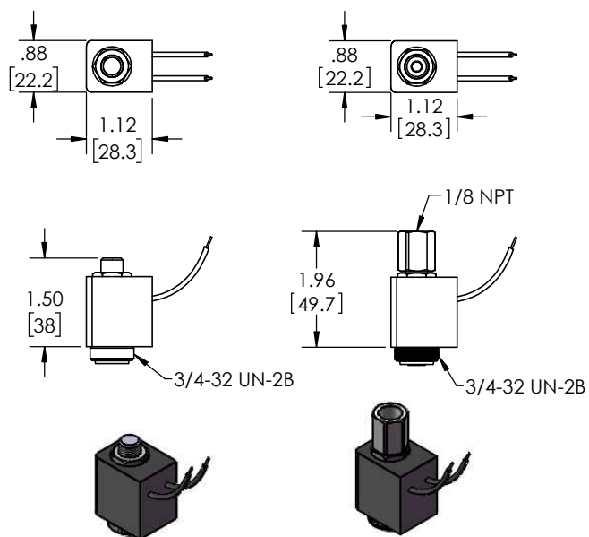
LEAD WIRE COIL
