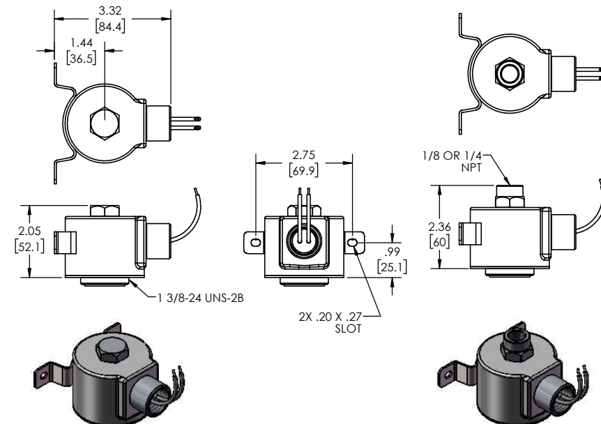
CONDUIT HOUSING WITH MOUNTING BRACKET
