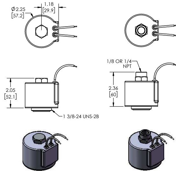
GROMMET HOUSING
