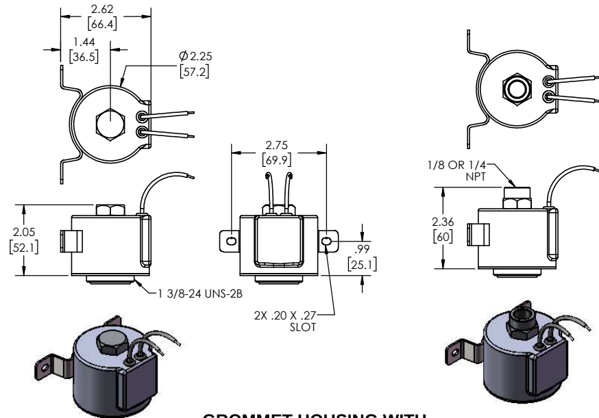
GROMMET HOUSING WITH MOUNTING BRACKET
