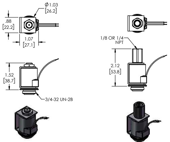
YOKE WITH LEAD WIRES
