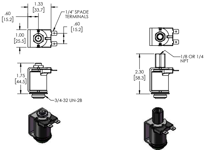
YOKE WITH SPADE COIL
