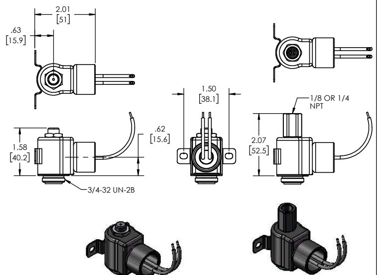
YOKE WITH LEAD WIRES
